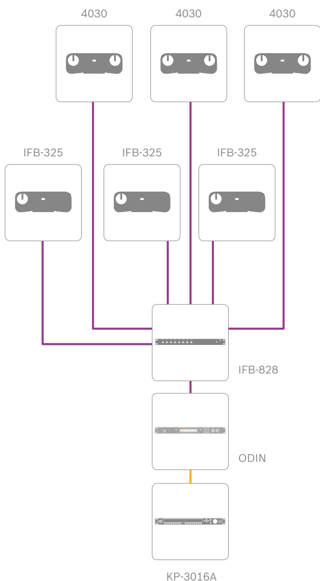
Digital Matrix IFB System
