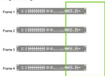
Four-frame ODIN system, single IFL ring
